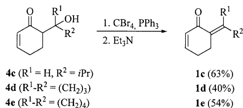
Scheme 4. Elimination of aldol adducts 4c–e under Appel conditions
