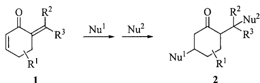
Scheme 1. Sequential Michael additions of two nucleophiles to dienones 1
