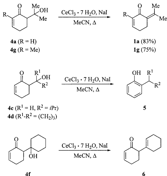
Scheme 3. Dehydration of aldol adducts 4 with \text{CeCl}_3 \cdot 7\text{H}_2\text{O}/\text{NaI}
