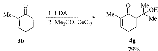
Scheme 2. \text{CeCl}_3 -mediated aldol reaction of cyclohexenones 3
